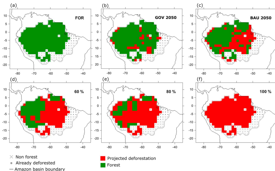
Figure 1. Deforestation scenarios. (a) Observed forest cover in 2003 when already 10% of the original forest extent is lost (gray dots). This land-cover map is used as baseline for control runs. (b) Governance (GOV) deforestation for 2050 reaching 20% of the original forest cover. (c) Business-as-usual (BAU) deforestation for 2050 reaching 45% of the original forest cover. (d–f) Deforestation reaching approximately 60, 80, and 100% of the original forest cover.
