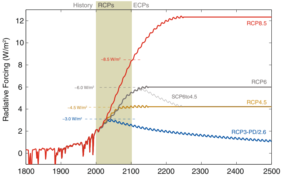
Fig. 4 Total radiative forcing (anthropogenic plus natural) for RCPs,—supporting the original names of the four pathways as there is a close match between peaking, stabilization and 2100 levels for RCP2.6 (called as well RCP3-PD), RCP4.5 & RCP6, as well as RCP8.5, respectively. Note that the stated radiative forcing levels refer to the illustrative default median estimates only. There is substantial uncertainty in current and future radiative forcing levels. Short-term variations in radiative forcing are due to both volcanic forcings in the past (1800–2000) and cyclical solar forcing—assuming a constant 11-year solar cycle (following the CMIP5 recommendation), except at times of stabilization
